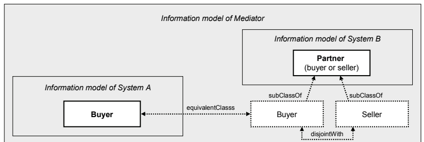
Figure 5-84 Mapping symbols of more specific/general concepts (bidirectional)
