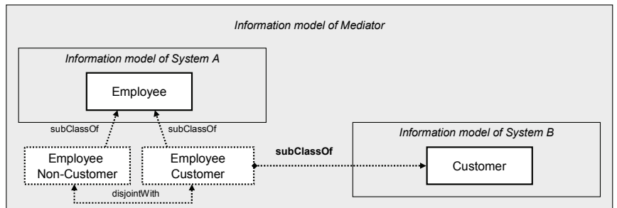
Figure 5-83 Mapping symbols of overlapping concepts (unidirectional)
