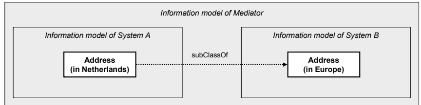
Figure 5-80 Mapping symbols of more specific/general concepts (unidirectional)
