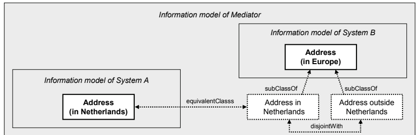
Figure 5-79 Mapping symbols of more specific/general concepts (bidirectional)
