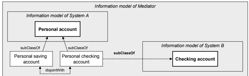
Figure 5-78 Mapping symbols of overlapping concepts (unidirectional)
