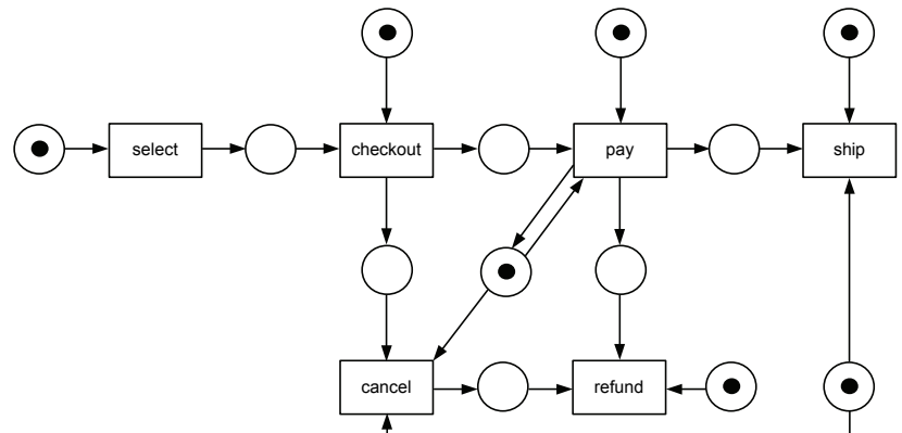
Figure A-177 Possible markings of the example in Figure 5-69
