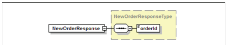
Figure B-190 XSD of message M 6 Create new order Response
