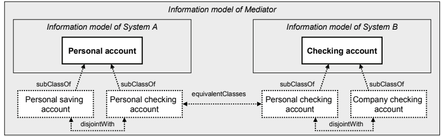
Figure 5-77 Mapping symbols of overlapping concepts (bidirectional)
