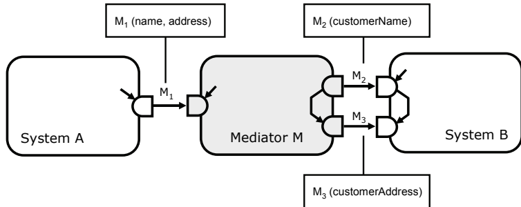
Figure 5-107 Defining a mediator that matches the send and received messages by the systems to be integrated
