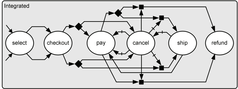
Figure A-180 The example from Figure A-179 after abstracting from the participating systems
