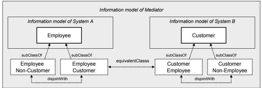
Figure 5-82 Mapping symbols of overlapping concepts (bidirectional)
