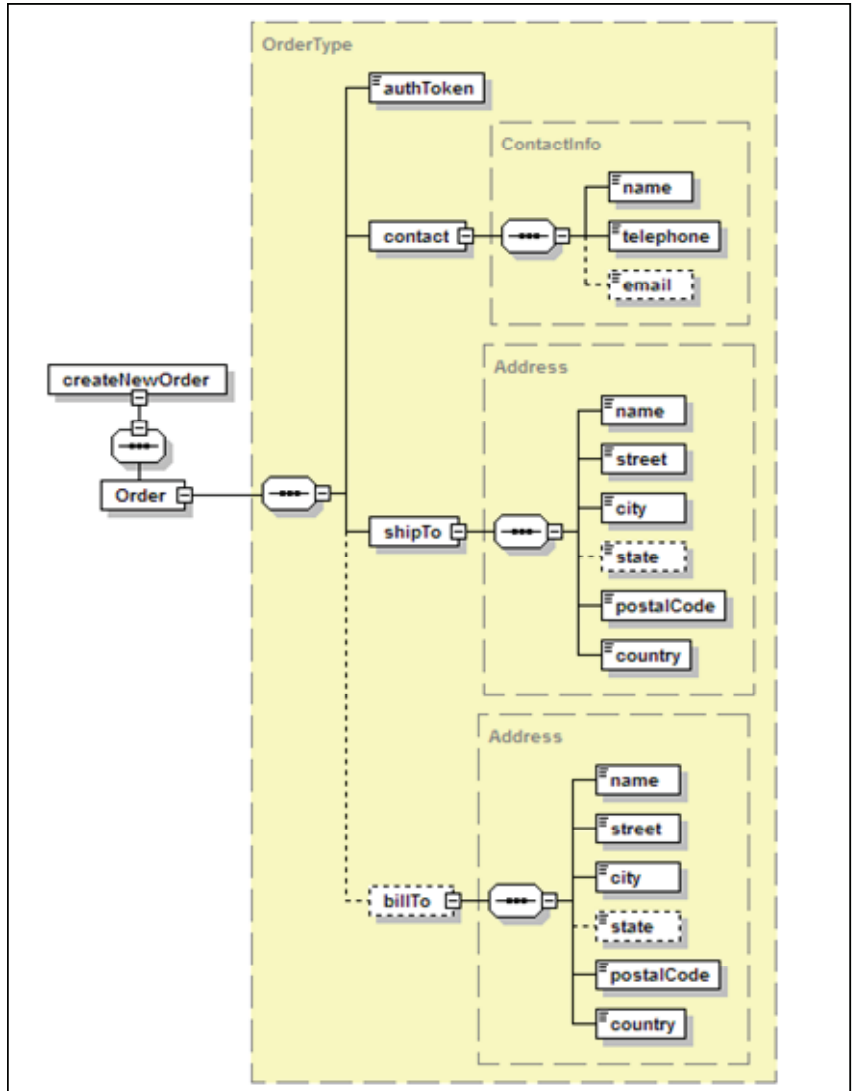
Figure B-189 XSD of message M 5 Create new order Request
