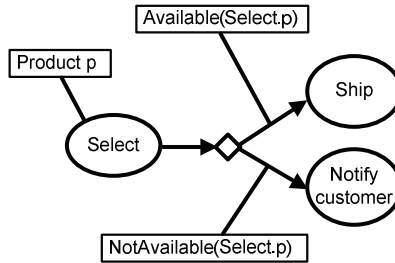
The causality relation for the actions Ship and Notify customer refer to the result of the action Select
