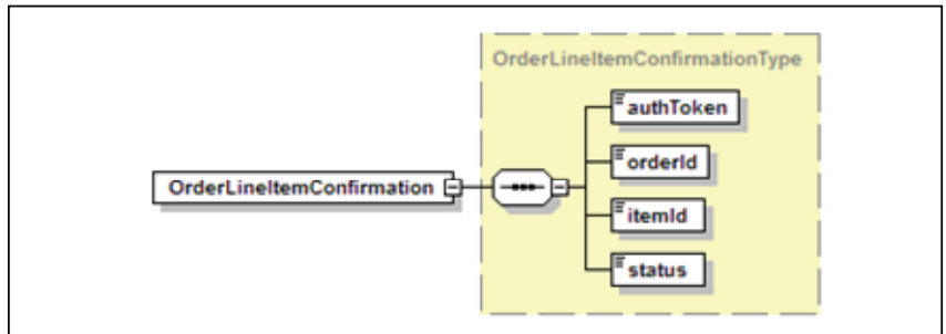
Figure B-194 XSD of message M 10 Confirm line item
