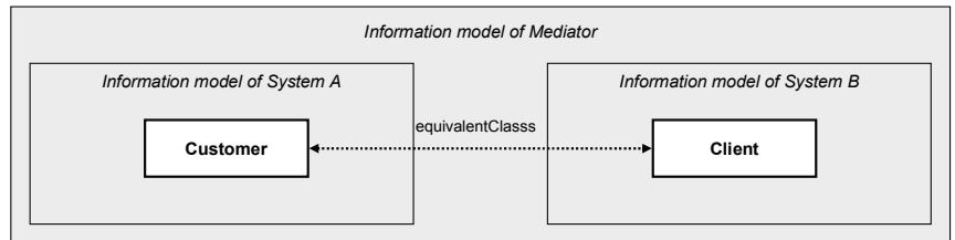
Figure 5-81 Mapping symbols of equivalent concepts
