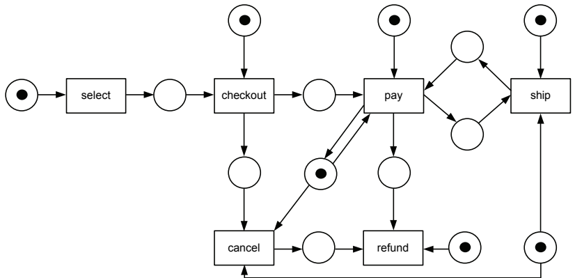
Figure A-182 The net corresponding to the behavior in Figure A-181
