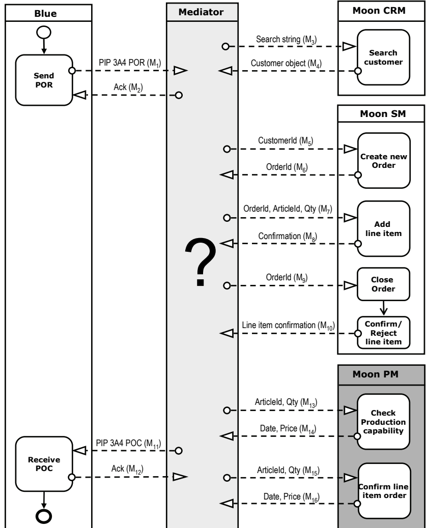
Figure 7-138 Blue's and Moon's systems
