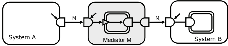
Figure 5-99 Splitting to multiple messages of the same type
