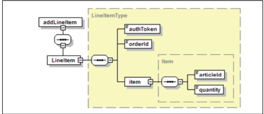
Figure B-191 XSD of message M 7 Add line item Request
