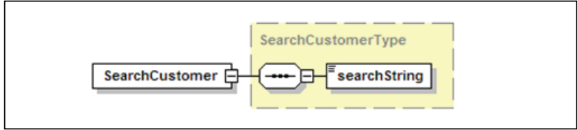
Figure B-187 XSD of message M 3 Search customer Request
