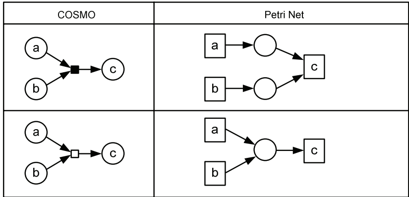
Figure A-168 Mapping conjunction and disjunction of conditions
