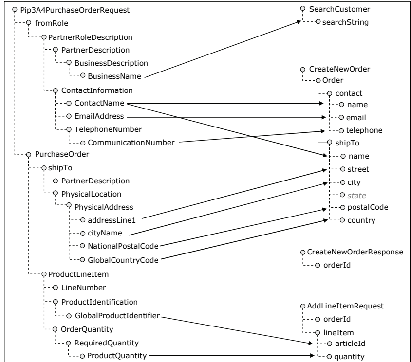
Figure 7-126 The mapping between the information PIMs of Blue and Moon
