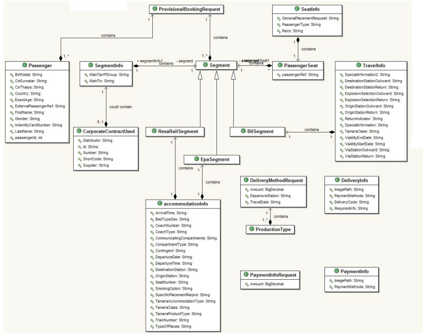
Figure C-205 The information model of ITTI
